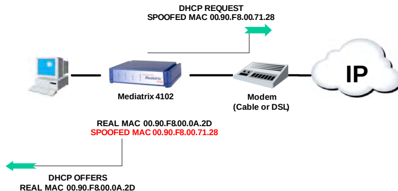
Figure 39: MAC Address Spoofing
