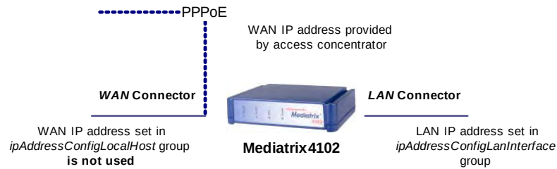
Figure 38: DSL Modem IP Addresses (PPPoE)
