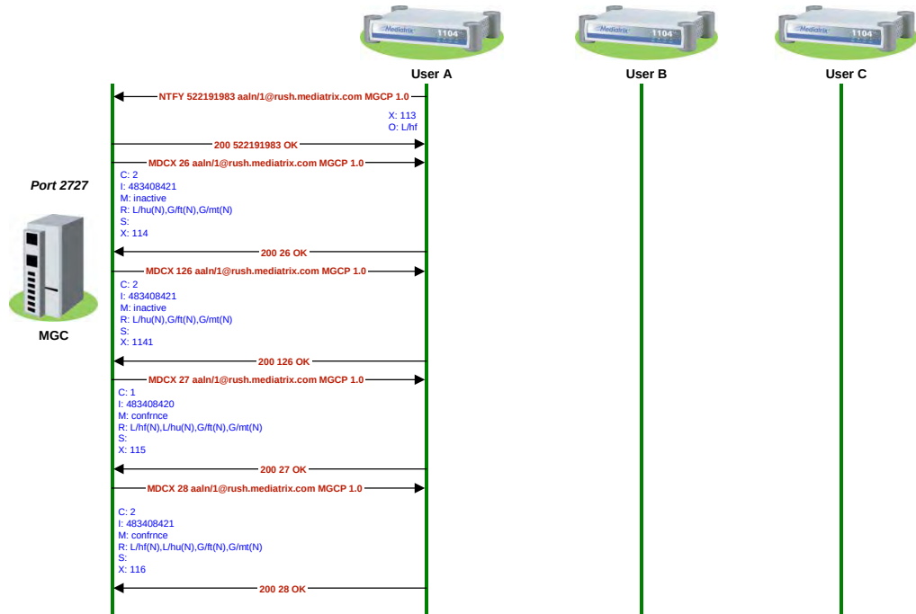
Figure 33: Conference Message Flow – Part 3
