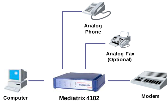
Figure 4: Single Computer Network Configuration
