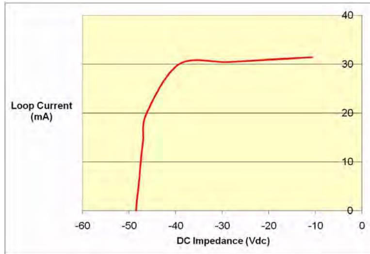
Figure 42: Loop Current vs Impedance – 32 mA
