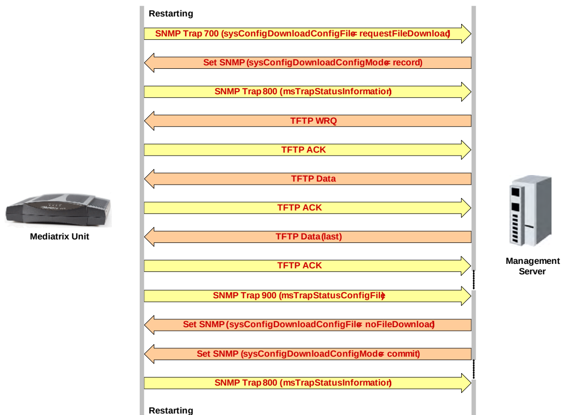
Figure 41: Configuration Sequence Update Using the Management Server
