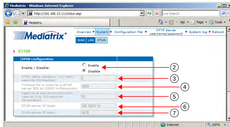
Figure 14: STUN Web Page
