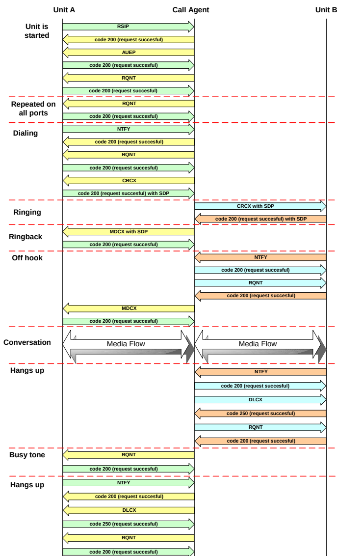
Figure 30: MGCP CALL Flow
