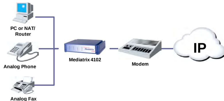
Figure 35: Mediatrix 4102 Residential Application Scenario
