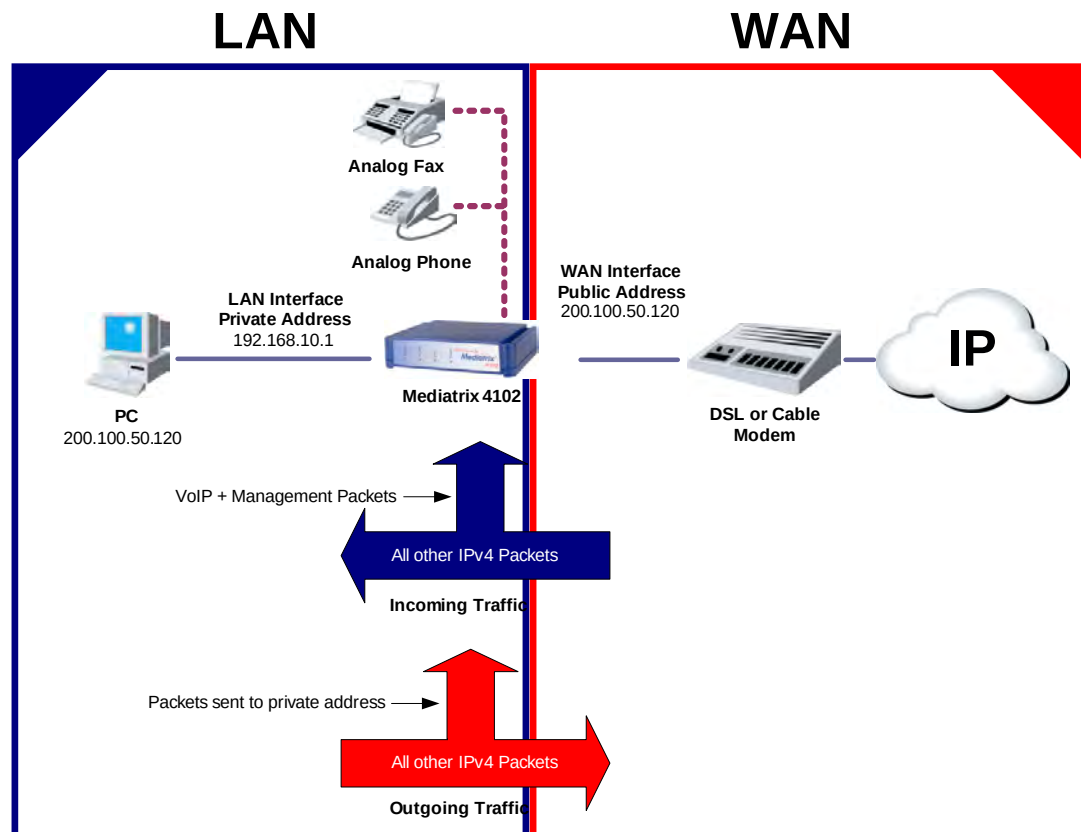
Figure 36: Transparent Address Sharing
