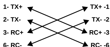
Figure 48: Crossover Connectivity
