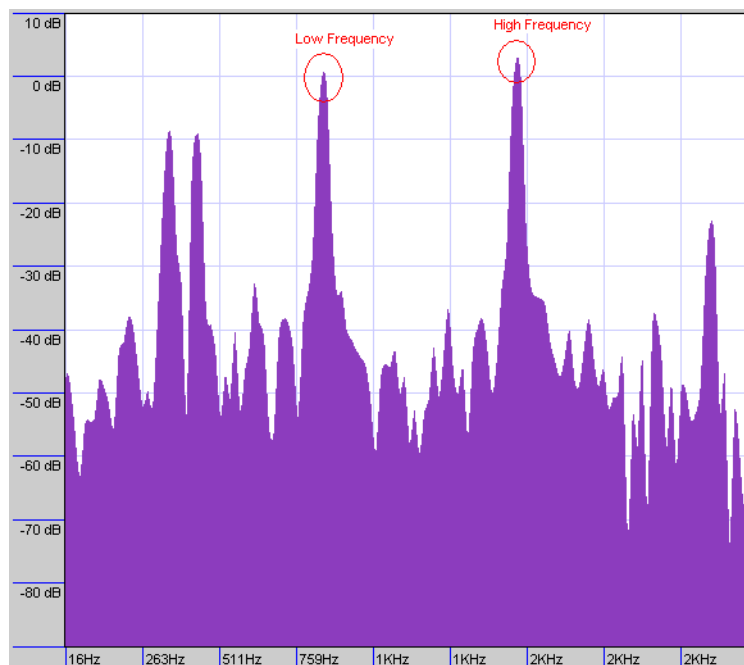
Figure 43: DTMF Detection Example
