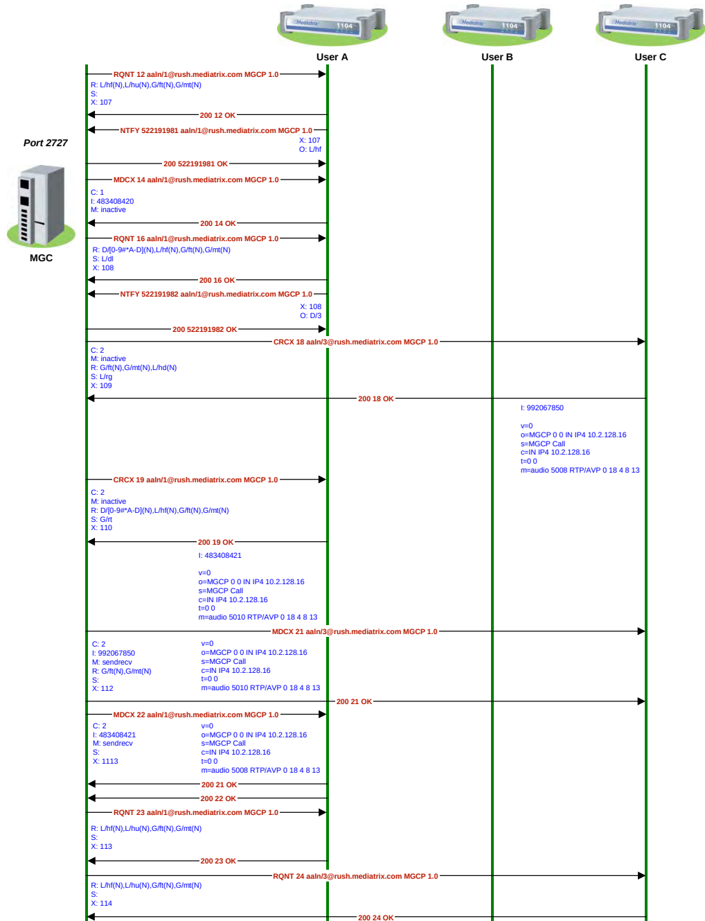
Figure 32: Conference Message Flow – Part 2
