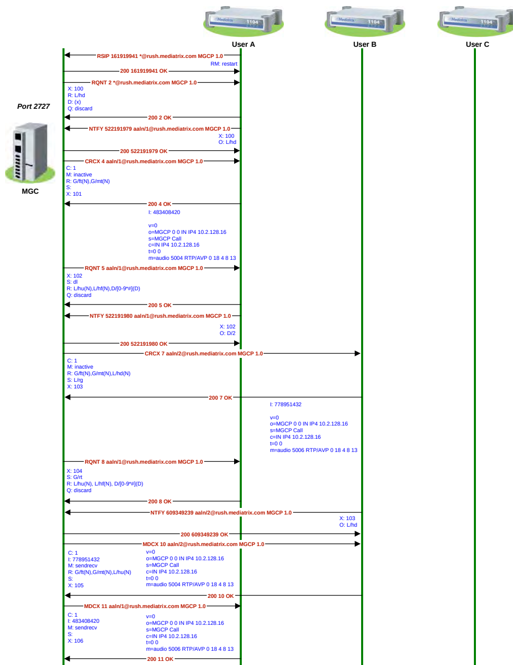
Figure 31: Conference Message Flow – Part 1
