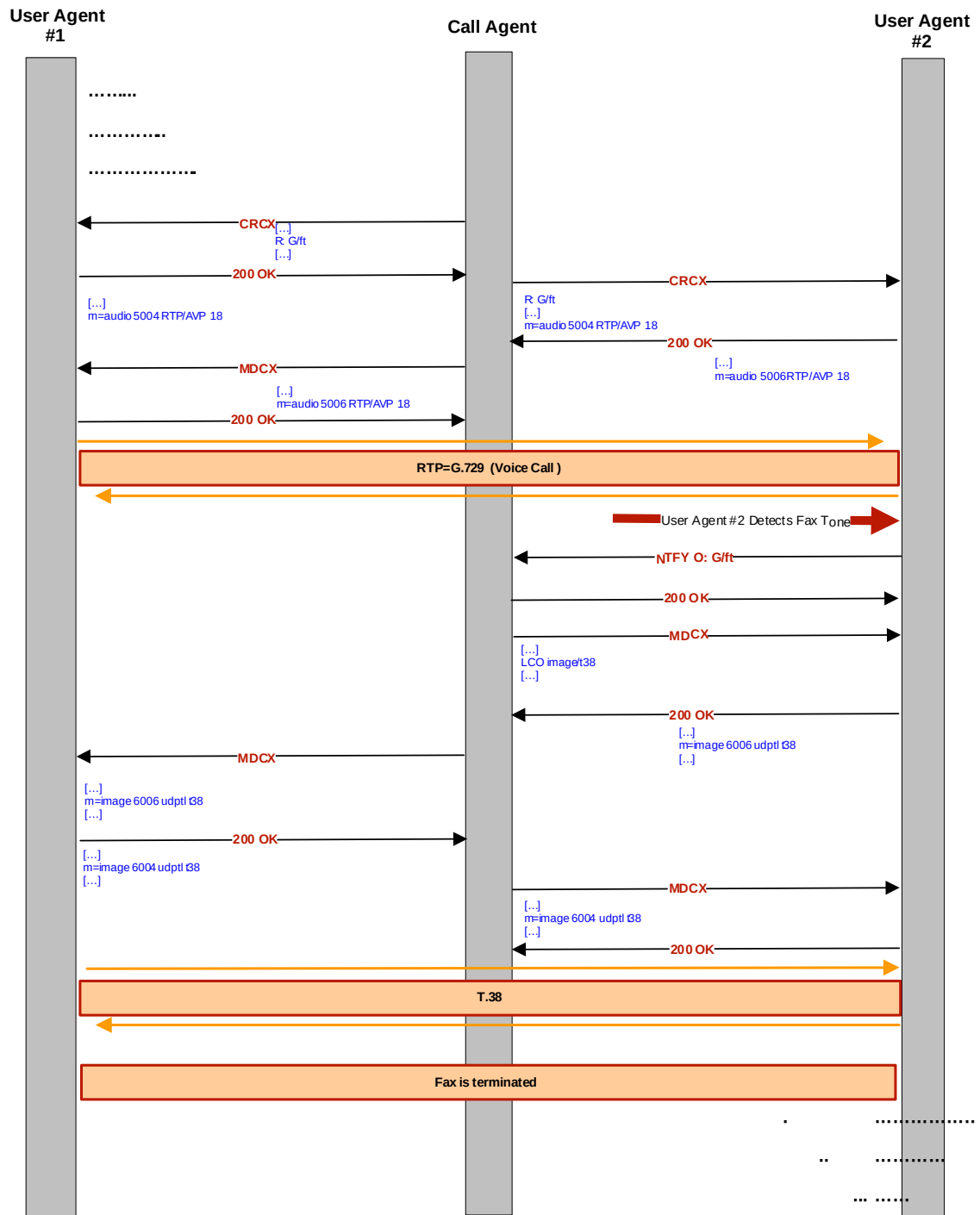
Figure 45: T.38 Fax Call Flow
