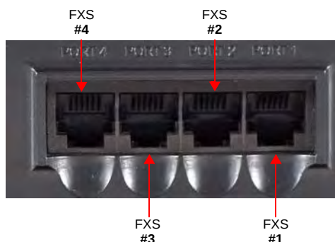
Figure 3: FXS Connectors Port Numbering Convention
