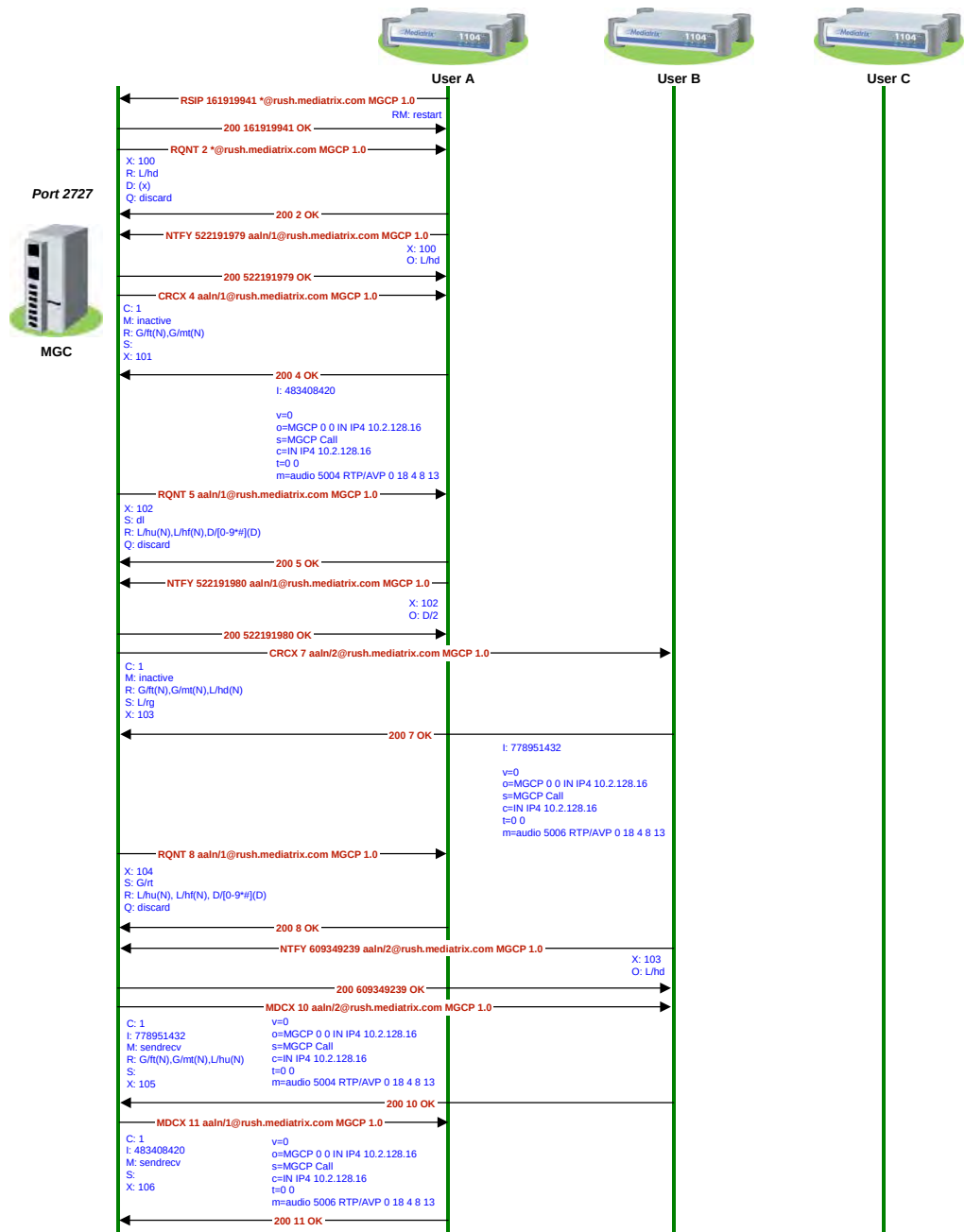
Figure 21: Conference Message Flow – Part 1
