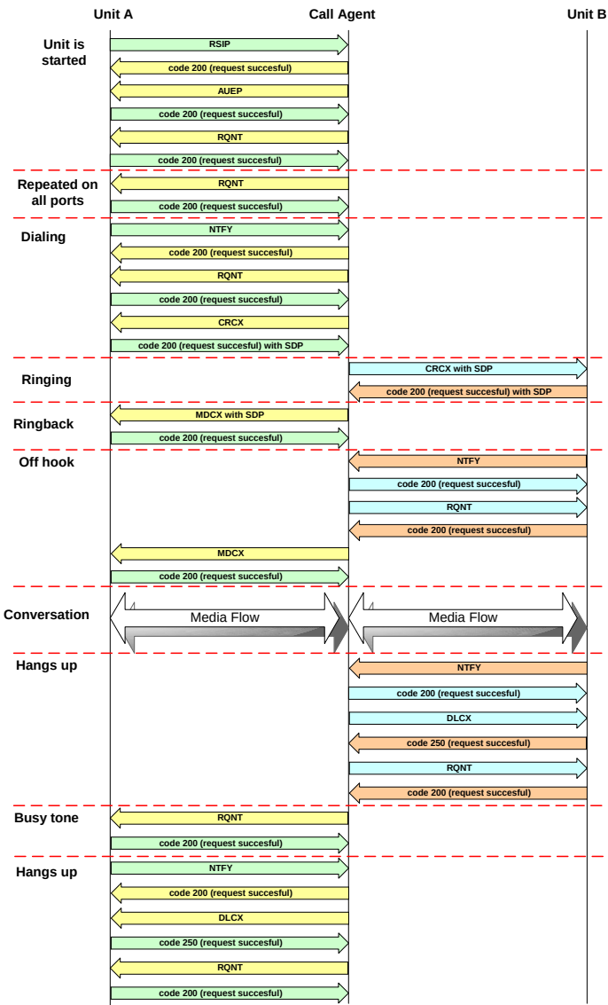
Figure 20: MGCP CALL Flow
