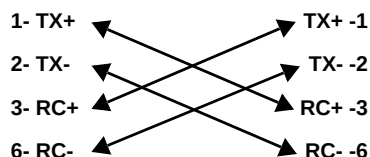
Figure 32: Crossover Connectivity
