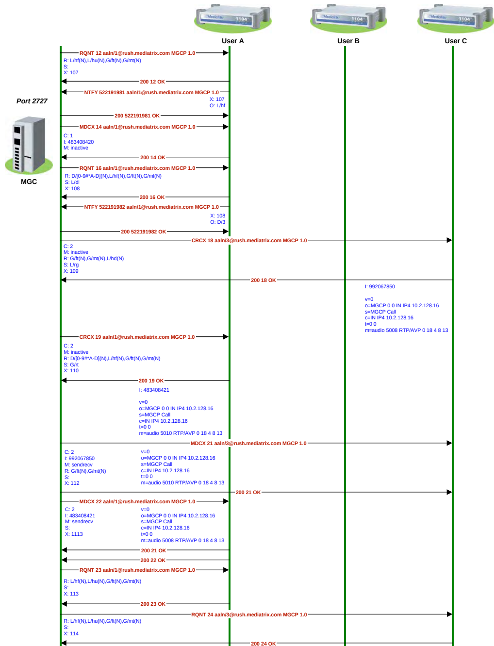
Figure 22: Conference Message Flow – Part 2
