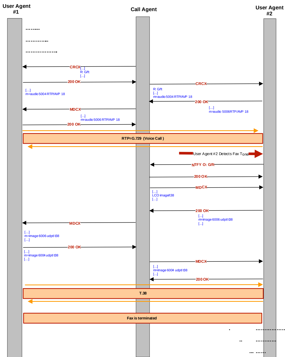
Figure 29: T.38 Fax Call Flow
