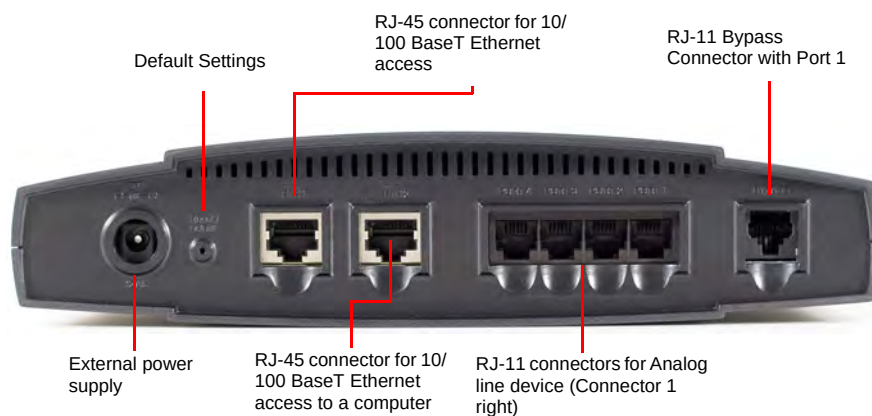
Figure 2: Back Panel Connectors
