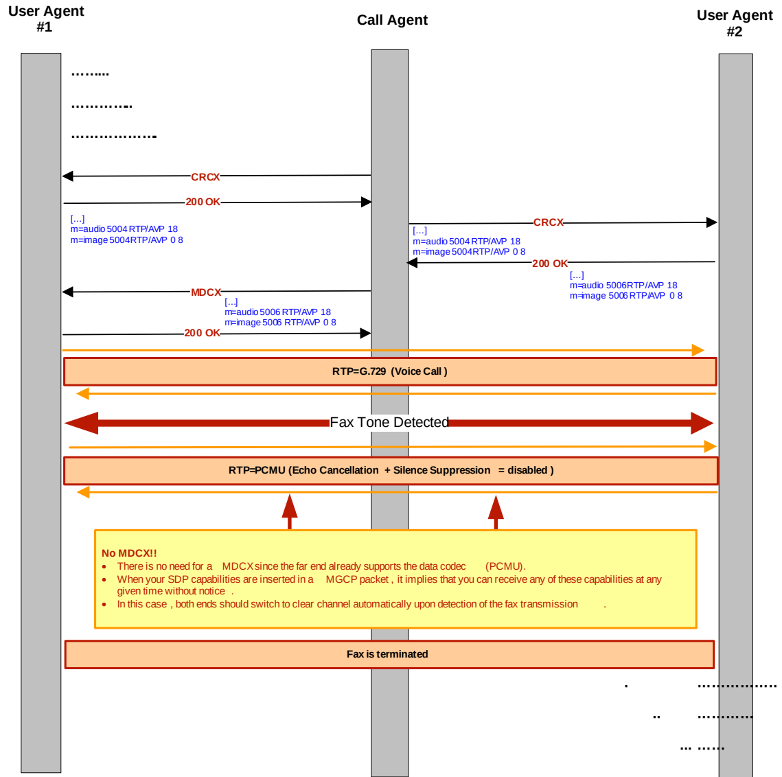
Figure 28: Clear Channel Fax Call Flow
