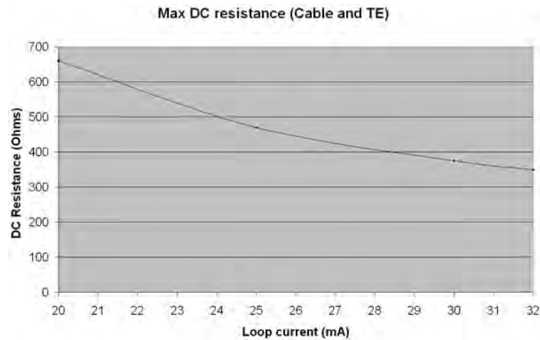
Figure 34: Max DC Resistance
