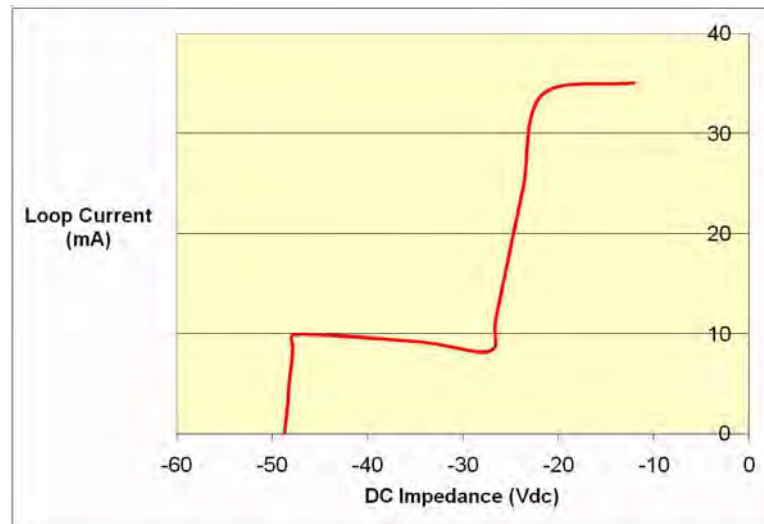
Figure 26: Loop Current vs Impedance – 32 mA
