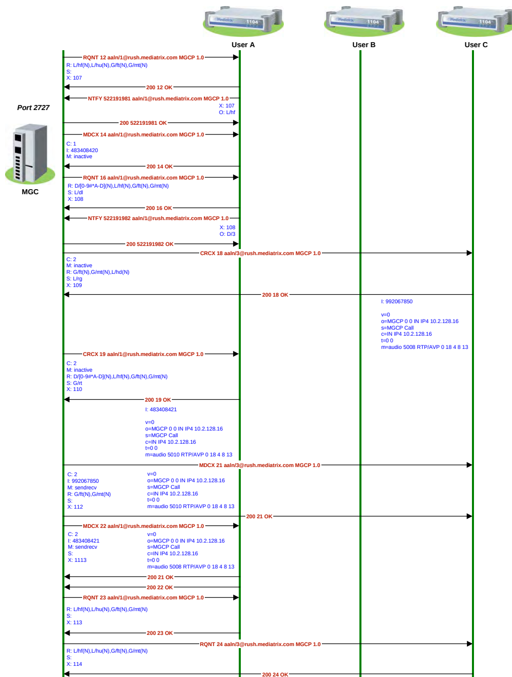
Figure 22: Conference Message Flow – Part 2
