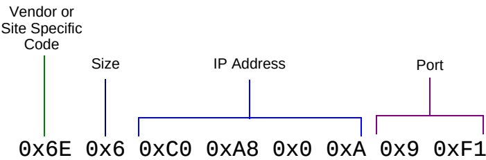
Figure 16: Example – Long Address String
