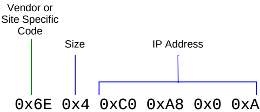
Figure 16: Example – Long Address String
