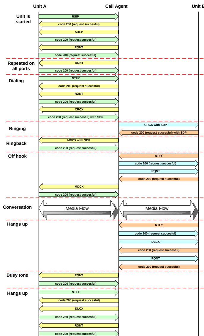
Figure 20: MGCP Call Flow
