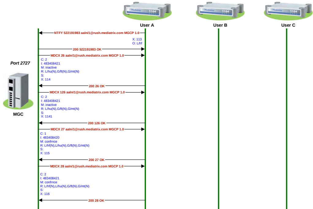
Figure 23: Conference Message Flow – Part 3
