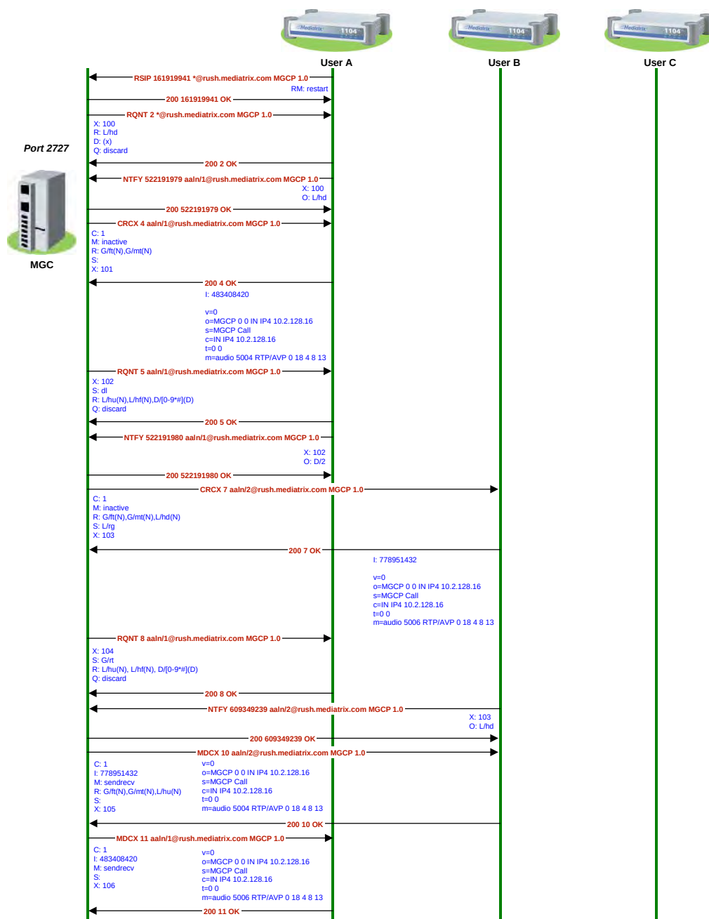
Figure 21: Conference Message Flow – Part 1
