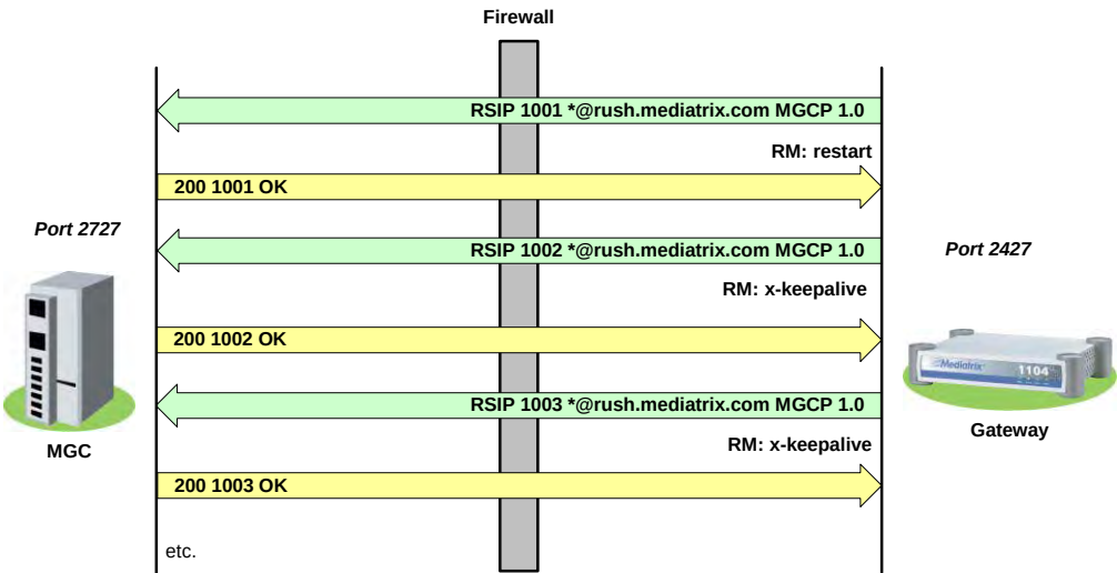
Figure 24: Firewall Message Flow
