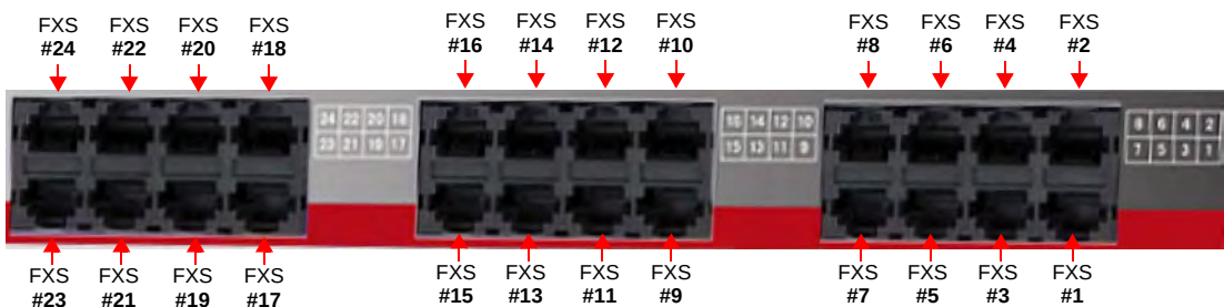
Figure 3: Mediatrix LP24 FXS Connectors Port Numbering Convention
